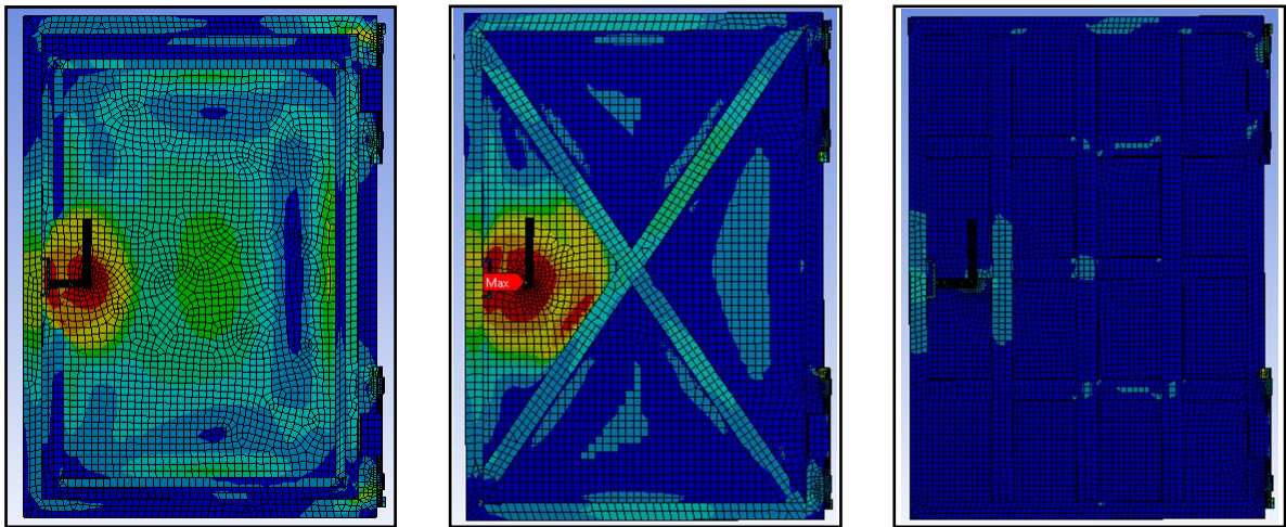
BIP RA stopping/door system blast response
